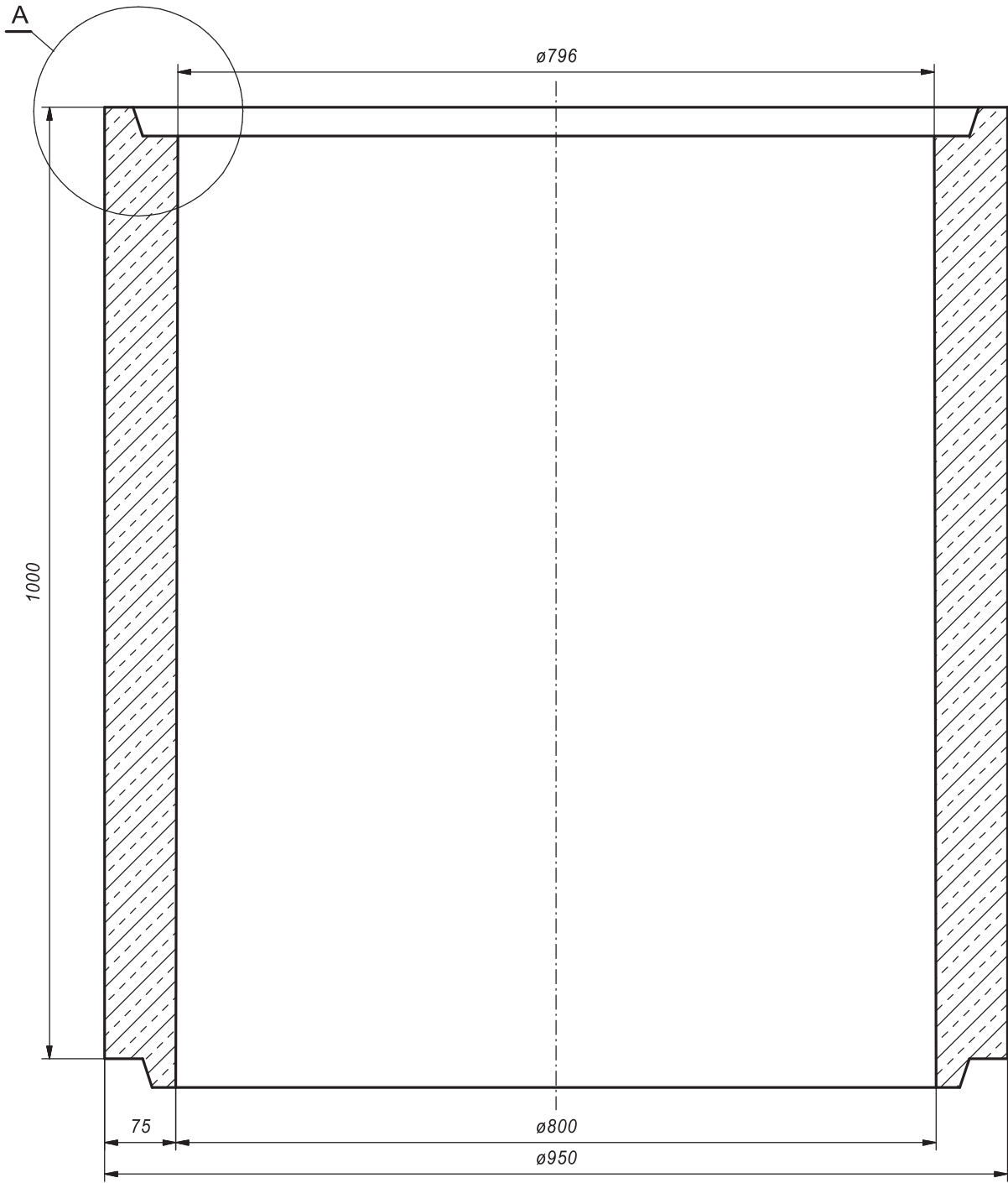
Section "A"
